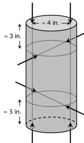
FIGURE 3. Shrinkage measurement locations.
